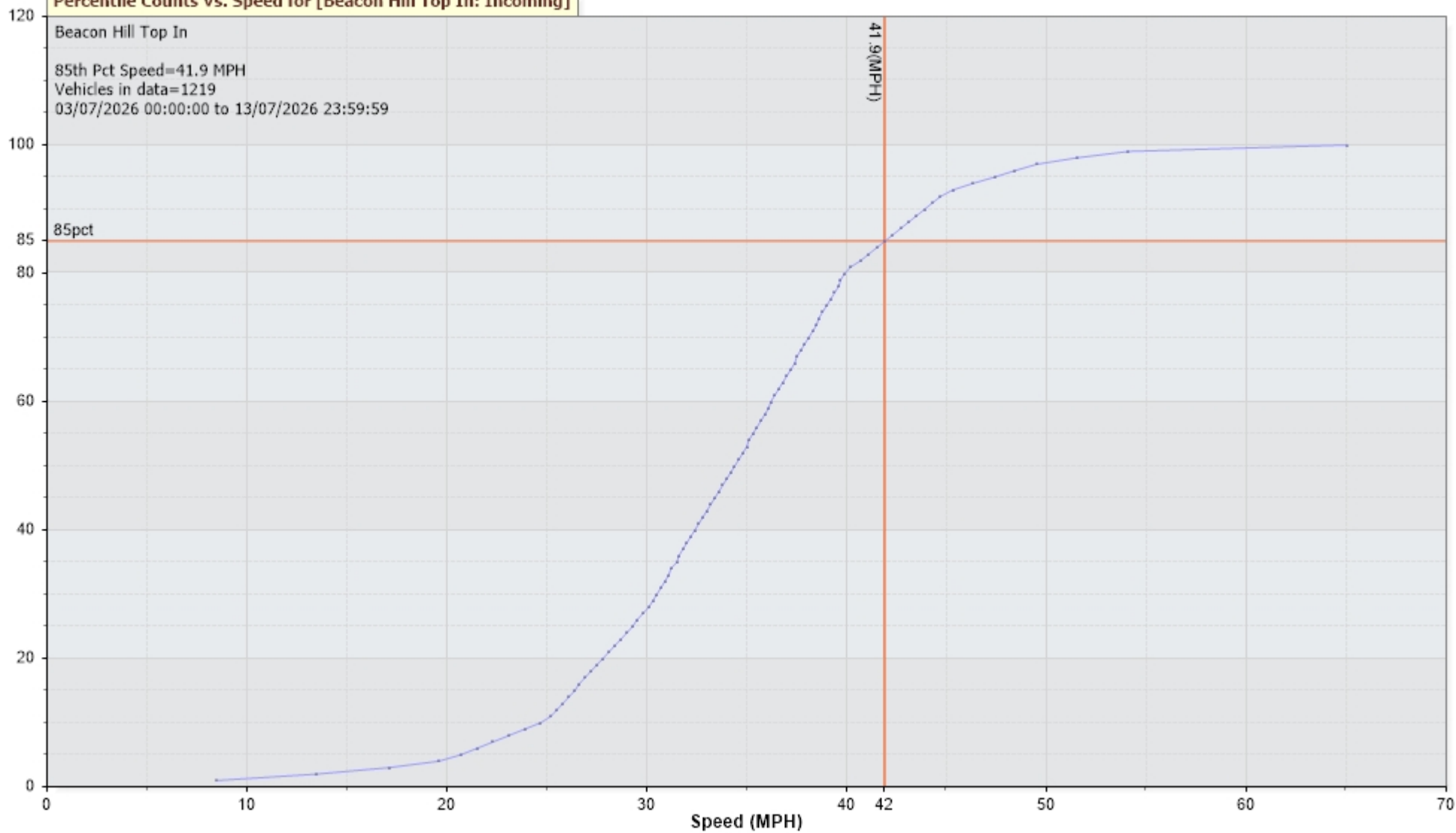
Percentile Counts Vs. Speed for [Beacon Hill Top In: Incoming]
