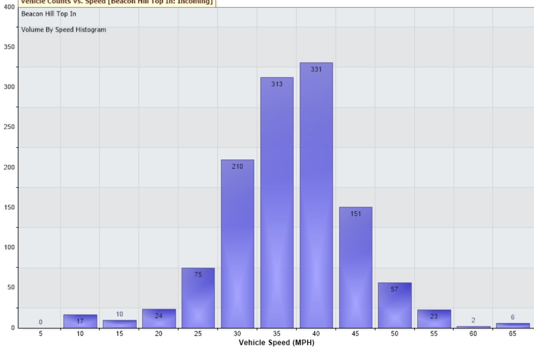
Vehicle Counts Vs. Speed [Beacon Hill Top In: Incoming]
