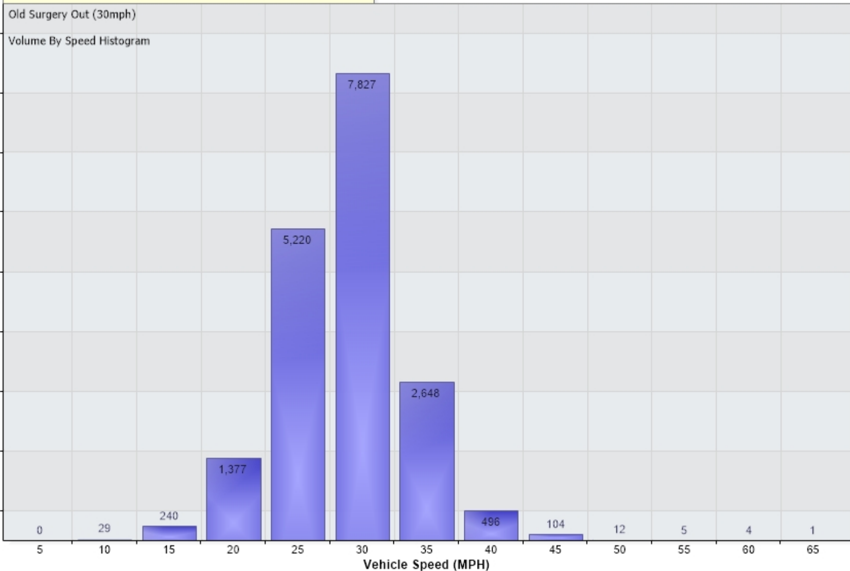
Vehicle Counts Vs. Speed [Old Surgery Out (30mph): Incoming]
