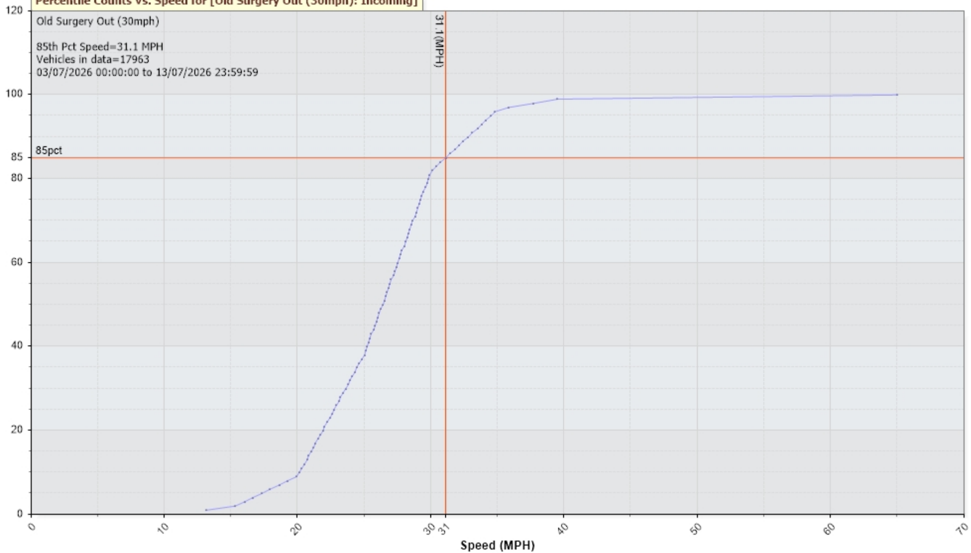
Percentile Counts Vs. Speed for [Old Surgery Out (30mph): Incoming]
